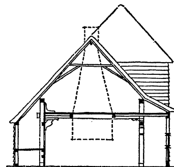
DWARSDOORSNED C-D.
