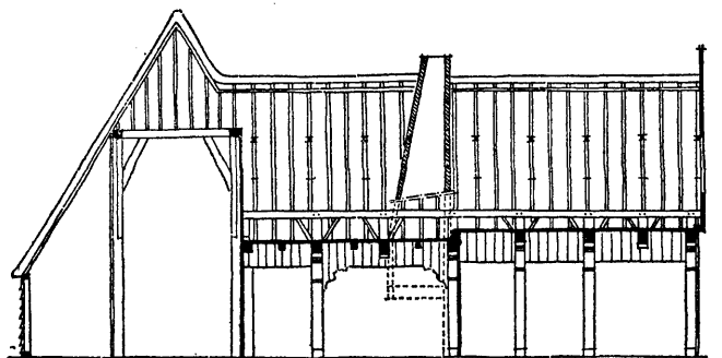
LANGSDOORSNED E-B.
