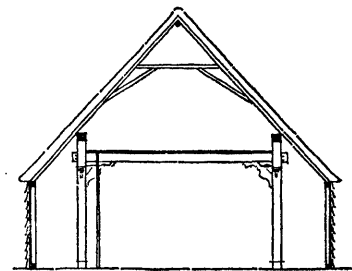
DWARSDOORSNED E-F.
